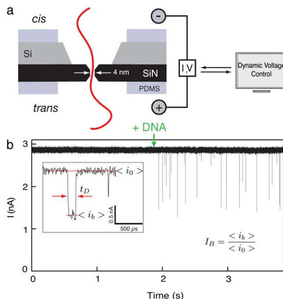
FIGURE 1 ( a ) Schematic illustration of a solid-state nanopore device for probing DNA translocation dynamics (not to scale). DNA molecules are driven through the nanopore by an applied voltage while the ion current of an electrolyte is measured. Dynamic voltage control is used to automatically unclog the pore when a molecule remains in the pore for > 5 s. Hourglass-shaped nanopores with diameters in the range 3 < d < 8 nm and effective thickness of \sim 10 nm were used (see text). ( b ) A typical ion-current trace for a 4-nm pore, before and after the introduction of 5 nM 400-bp DNA to the cis chamber (green arrow). The transient current-blockade events correspond to single-molecule translocation of DNA. The inset displays a magnified translocation event, in which the relevant parameters used in this article are defined.
