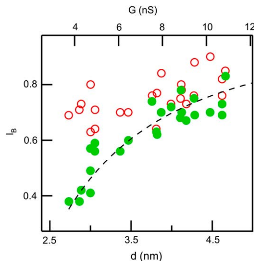
FIGURE 6 I_{BL} (green) and I_{BH} (red) values for a series of 25 nanopores with different diameters in the range 2.7–4.6 nm, measured using a 400-bp fragment (each I_B pair is based on a histogram of >1500 events, as in Fig. 4). The dashed line is the theoretical I_B curve based on Eq. 1, with a = 2.2 nm, showing excellent agreement with I_{BL} and clearly deviating from I_{BH} .
